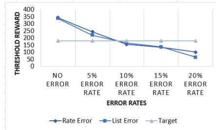
Fig. 11. Total obtainable reward with HPN
