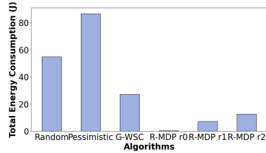
Fig. 14. Total energy consumption by algorithm
