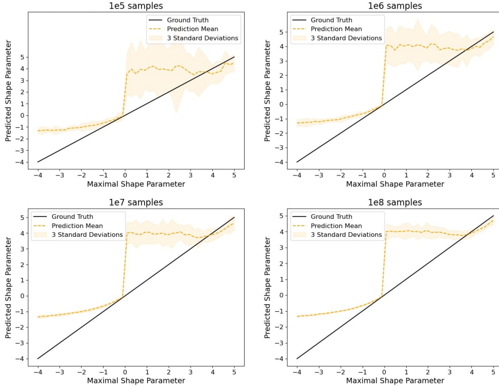
Figure 2: Estimation of the shape parameter of the marginal by direct application of POT. We utilize the Pickands estimator as our estimator of choice.
