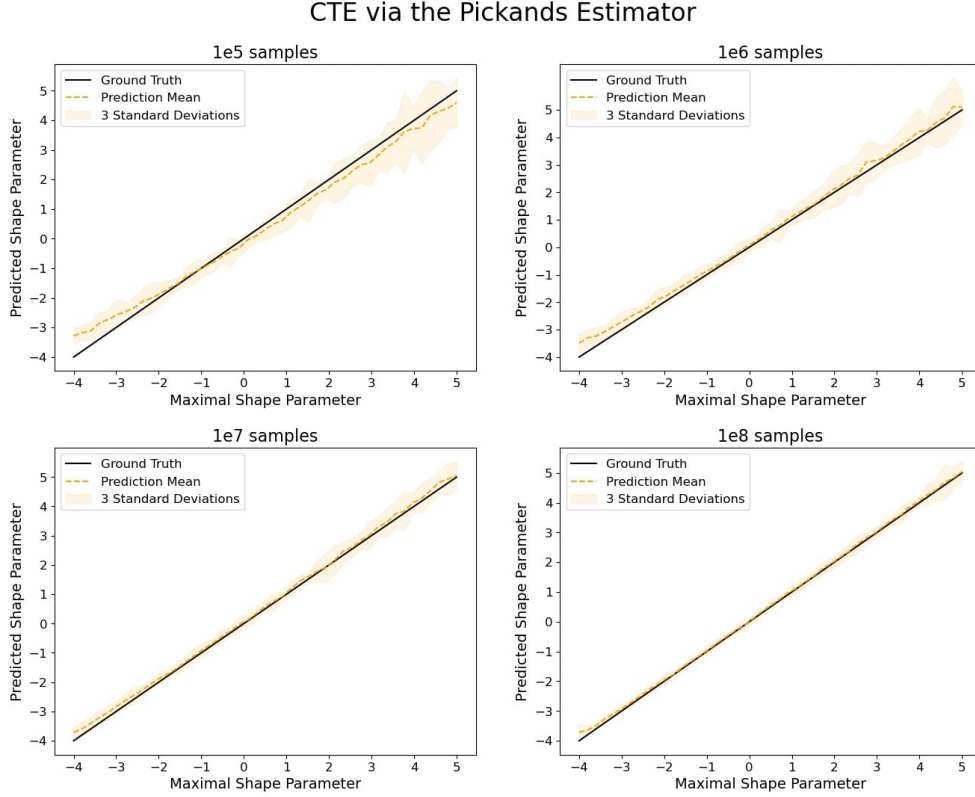
Figure 3: Estimation the shape parameter of the marginal using CTE. We utilize the Pickands estimator as our estimator of choice.
