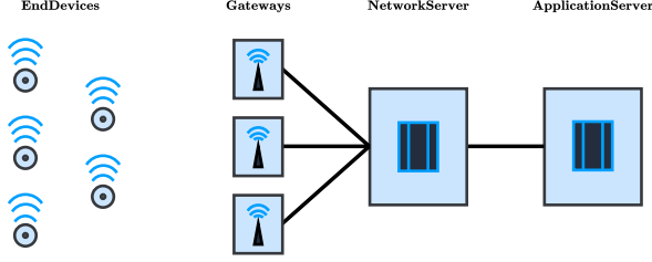
Fig. 1: LoRaWAN architecture.
