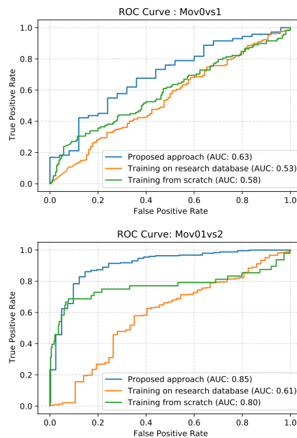
Figure 3: Receiver operating characteristic curves (ROC) for the detection of severe (mov01vs2) and moderate (mov0vs1) motion in 3D T1w MRIs.
