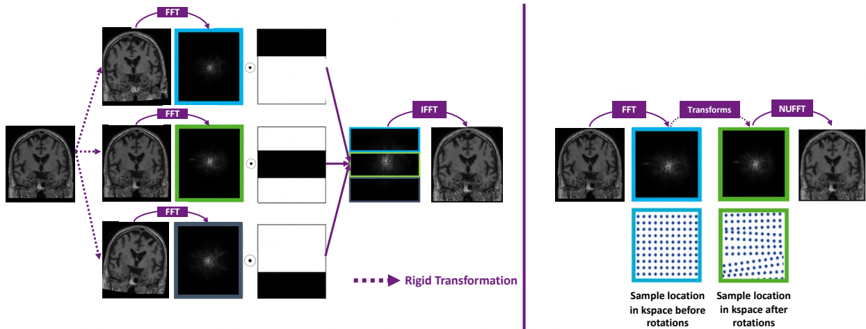
Figure 1: Left: Image-based motion simulation. (1) Nt rigid transformations of the motion-free image are applied (here Nt = 2 ), (2) Fast Fourier transform (FFT) of the original and Nt transformed images, (3) Concatenation of the Nt + 1 blocks to create a new k-space, (4) Inverse FFT (IFFT) to obtain the motion corrupted image. Right: k-space based motion simulation. (1) FFT of the motion-free image. (2) Transformation (rotation + translation) for each point of the time course. (3) Non uniform FFT (NUFFT) to reconstruct the corrupted image (because of the non uniform sample spacing due to the rotation in the k-space).
