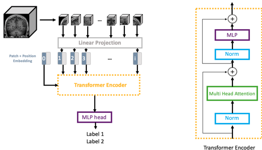
Figure S3: Architecture of the Vision Transformer (ViT) with the transformer encoder introduced by (Dosovitskiy et al., 2020).
