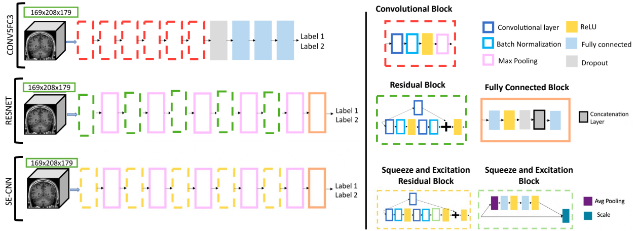
Figure S4: Architecture of the three CNNs trained in our study : the Conv5 FC3, the ResNet and the SECNN with the Squeeze and Excitation Residual blocks.
