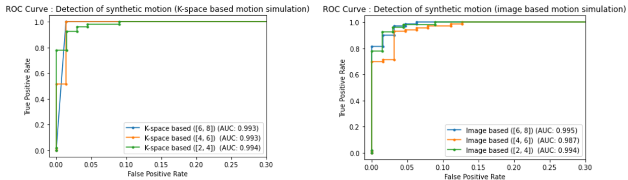
Figure S5: Receiver operating characteristic (ROC) curves for the detection of synthetic motion on the research dataset for various rotation and translation values with the image and k-space based methods.
