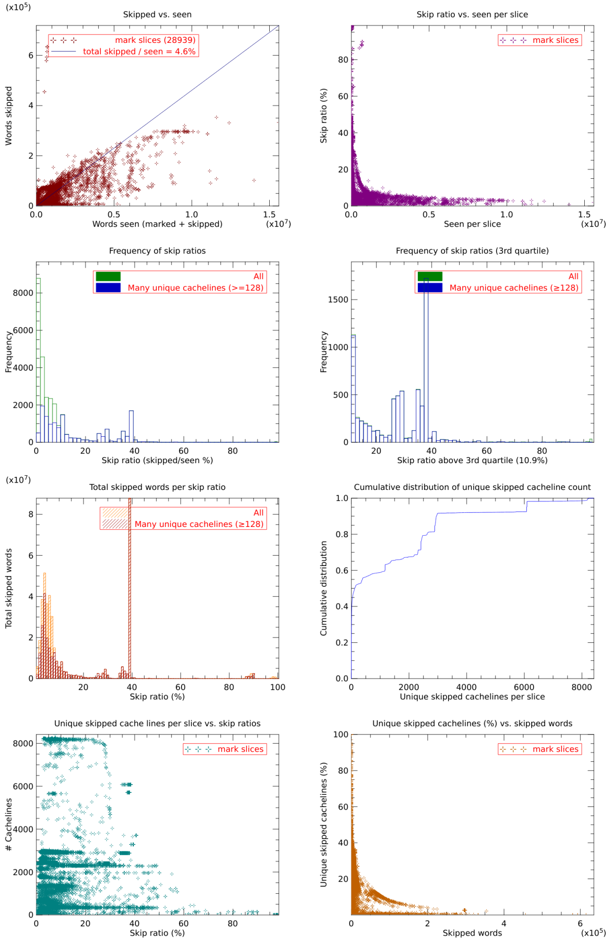
Figure 1: coq_mathcomp_no_native
