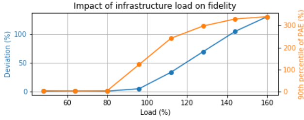
Fig. 4: High-level (blue) and low-level (orange) indicators of emulation fidelity (y-axis) vs. link load (x-axis).
