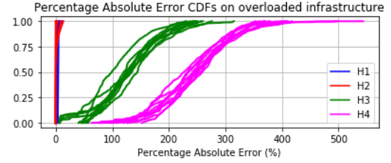
(b) CDFs of the percentage absolute errors (PAE). The blue plots correspond to the CDFs of locally emulated links in host H1 ; the red, green, and magenta to the CDFs of links overlay emulated between hosts H2 and H1 , hosts H3 and H1 , and hosts H4 and H1 respectively.
