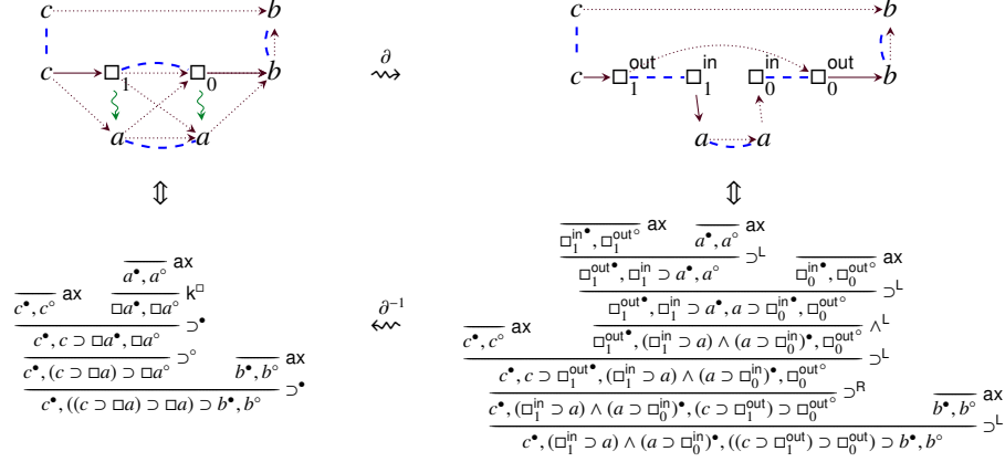
Fig. 8. A K-arena net \mathcal{G} with associated formula (c \wedge ((c \supset \Box a) \supset \Box a) \supset b) \supset b , its corresponding arena \partial(\mathcal{G}) , the LCK _\ell^\circ -derivation associated to \mathcal{G} and the LI _\ell^\circ -derivation associated to \partial(\mathcal{G})
