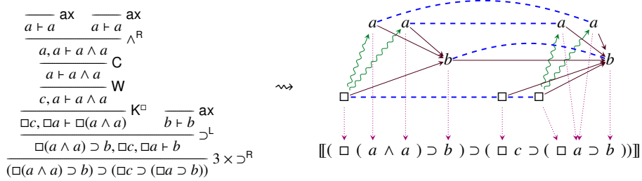
Fig. 1. A sequent calculus derivation of the formula (\Box(a \wedge a) \supset b, \Box c, \Box a) \supset b and its corresponding combinatorial proof
