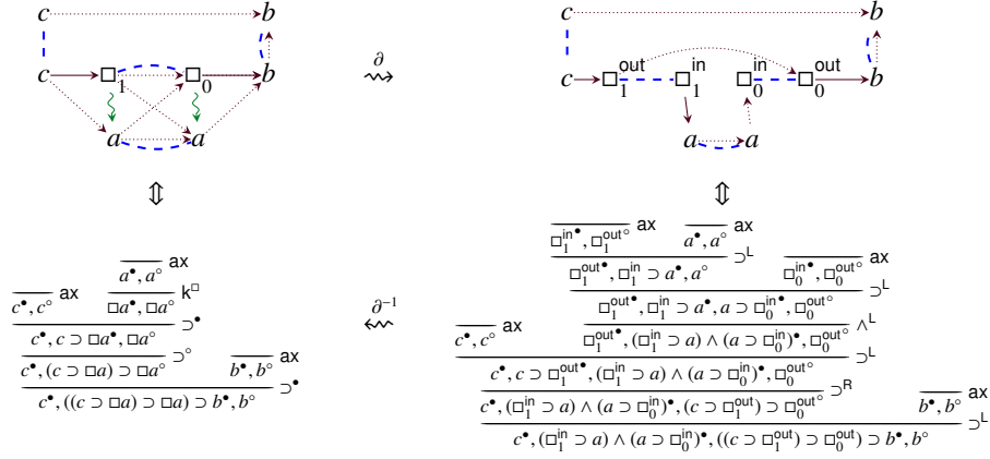
Fig. 8. A K-arena net \mathcal{G} with associated formula (c \wedge ((c \supset \Box a) \supset \Box a) \supset b) \supset b , its corresponding arena \partial(\mathcal{G}) , the LCK ℓ ∘ -derivation associated to \mathcal{G} and the LI ℓ ∘ -derivation associated to \partial(\mathcal{G})
