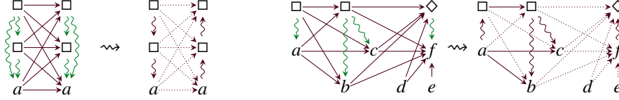
Fig. 5. The arenas of the sequents \vdash \Box\Box a \supset \Box\Box a and \Box a \supset \Box(b \wedge c), d \vdash \Diamond(e \supset f) and the corresponding graphs obtained by replacing the \rightsquigarrow -edges with \rightsquigarrow_{\partial} -edges.
