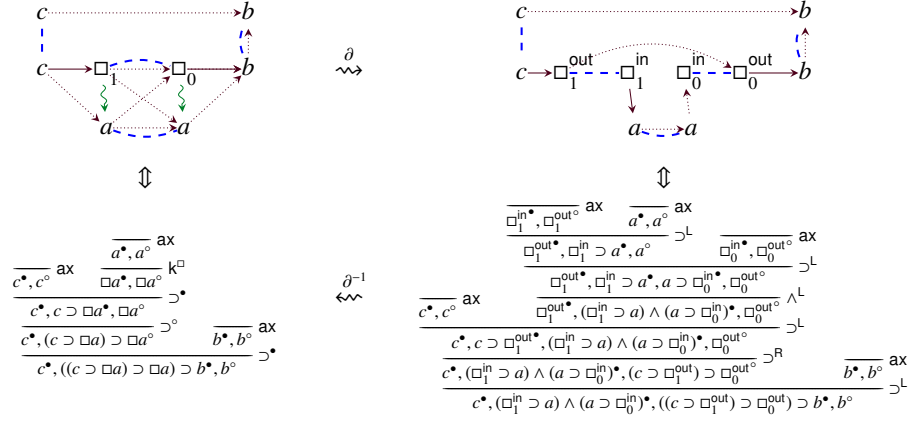
Fig. 8. A K-arena net \mathcal{G} with associated formula (c \wedge ((c \supset \square a) \supset \square a) \supset b) \supset b , its corresponding arena \partial(\mathcal{G}) , the \text{LCK}_\ell^\circ -derivation associated to \mathcal{G} and the \text{LI}_\ell^\circ -derivation associated to \partial(\mathcal{G})
