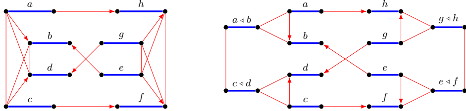
■ Figure 5 Left: The relational RB-prenet for Q in (10) and \Gamma_Q in (11). Right: A simplification of the tree-like RB-prenet in Figure 4.
