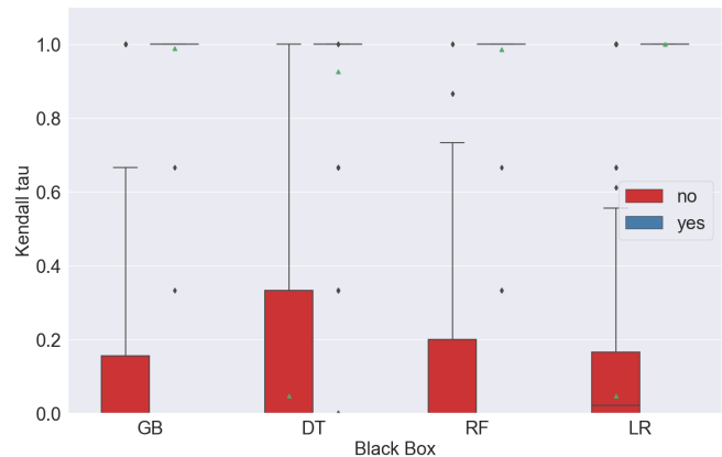
Figure 3: Average Kendall’s rank correlation coefficient of the LS_{APE} ’s explanations computed on 100 instances for 7 datasets and 4 “glass” black-box models across the oracle’s outcomes.
