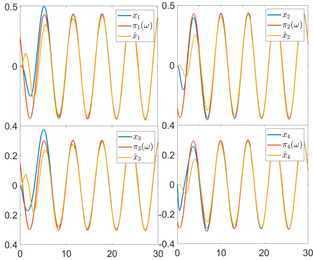
Fig. 2. Simulation results for Example 1. Initial conditions: x_i(0) = 0 ; \omega_1(0) = 0.1, \omega_2(0) = 0, \dot{\omega} = 0 . Coefficients: k_1 = k_2 = 3, k_3 = 0.6, a_1 = 0.6, a_2 = 2 .
