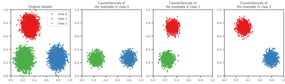
Figure 2: Comparison of the examples/counterfactuals distributions for synthetic data. All graphics represent the projection of the examples or counterfactuals on the first two dimensions of the examples space ( \mathbb{R}^8 ). The graphic on the left represents the original dataset. The three other graphics represent counterfactuals generated from the examples of the test set belonging to each class. For this three rightmost graphics, the same examples have been used to generate counterfactuals with the two other classes. The color/shape of the point represents a class information: the class an example belongs to (graphic on the left) and the class requested for counterfactual generation (3 graphics on the right).
