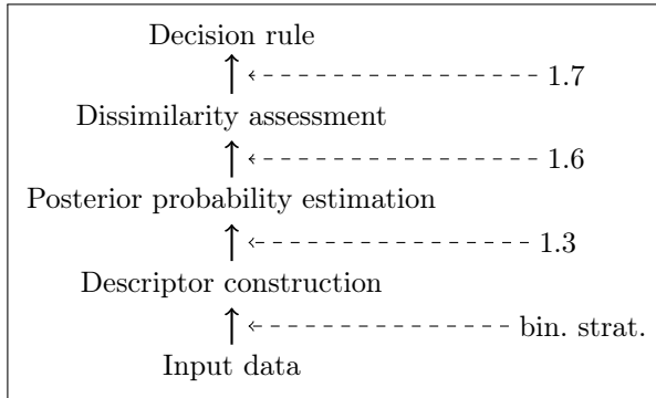
Fig. 1.1: High-level flowchart of investigated algorithm.
