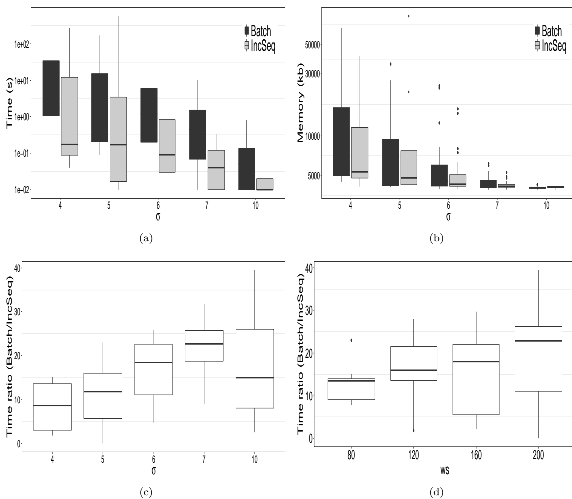
Figure 3: Comparison of processing time (logarithmic scale) and memory usage with respect to the support threshold \sigma (with ws < 25 ) and the size of the sliding window ws . (c) and (d) represent the respective computing time ratio of Batch to INCSEQ on the same dataset.
