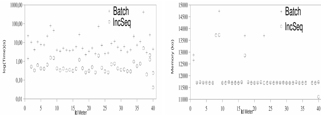
Figure 4: Comparison of computation time (left) and memory usage (right) when mining the power consumption streams.
