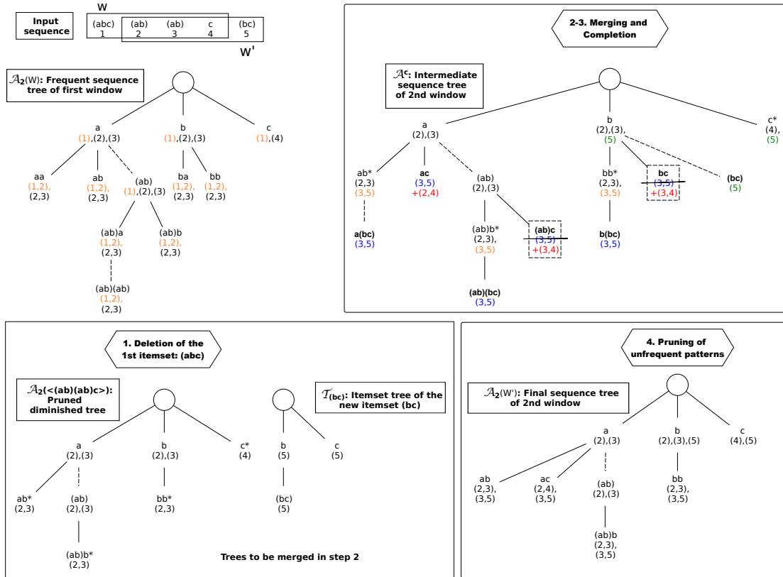
Figure 2: Successive steps for updating the tree of frequent patterns upon the arrival of itemset (bc) in the window W = \langle (abc)(ab)(ab)c \rangle .
