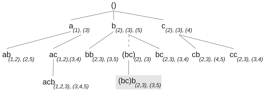
Figure 1: Example of a tree of frequent sequential patterns ( \sigma = 2 )
