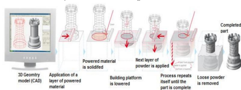
Fig. 1. Additive manufacturing process. Source [7].
