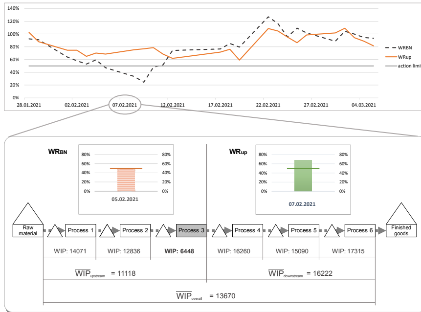
Fig. 3. The developed controlling instrument.
