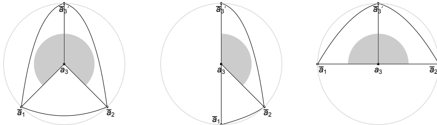
Figure 2: Three configurations where a_3 \in \langle a_1, a_2, a_3 \rangle together with their (local) contribution depicted in gray. All can be encoded using the same sum [\bar{a}_1, \bar{a}'_3] \oplus [\bar{a}_2, \bar{a}'_3] (as in \Sigma'(a_3) ).
