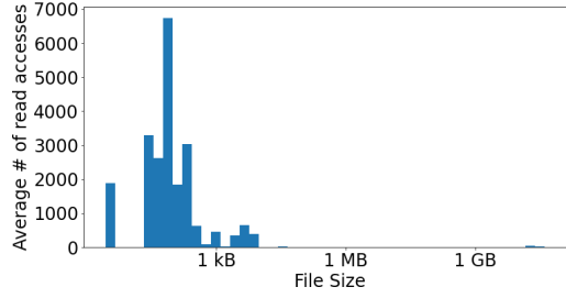
Figure 2: File popularity distribution.
