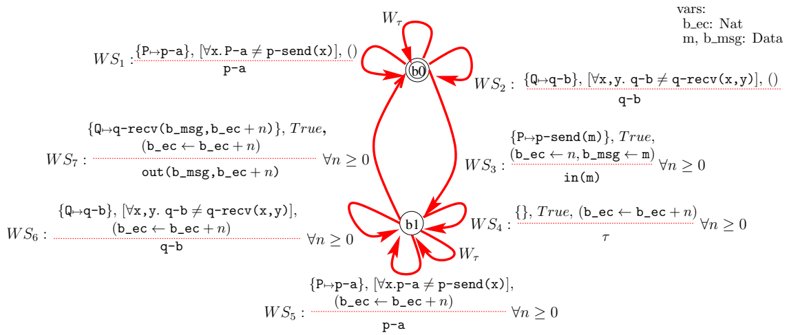
Figure 6: Weak Open Automaton of the Specification
