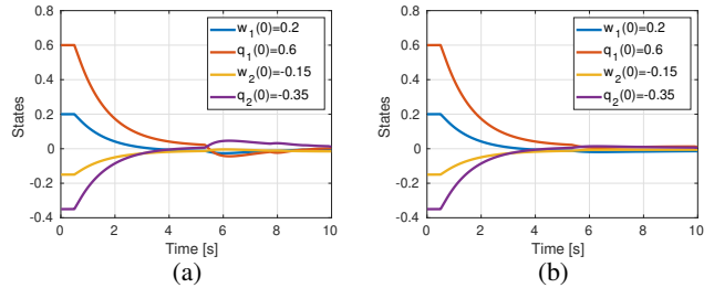
Fig. 1: Simulation for (a) input and (b) measurement delays
