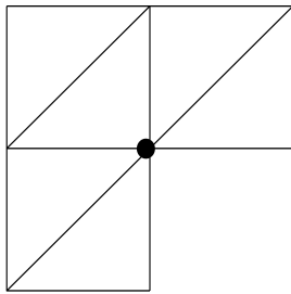
Figure 2: Uniform triangular mesh on the L-shape domain.
