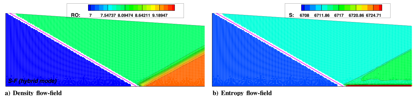
Fig. 10 Regular shock reflection: hybrid S-F computations (fitted shock is depicted using pink solid line).
