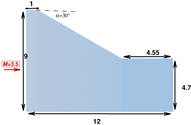
Fig. 12 Mach reflection: freestream conditions, domain, and background grid ( 232 \times 102 cells).
