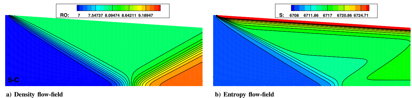
Fig. 9 Regular shock reflection: S-C computation.
