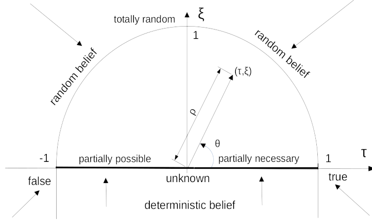
Figure 6: Representation of partial truth (\tau, \xi) \in \mathcal{R}^2 , with \tau \in [-1, 1] and \xi \in [0, 1] , in relation with necessity and possibility. If \xi = 0 (deterministic belief) the belief is entirely deterministic, which corresponds to a real grounding. If \tau^2 + \xi^2 = 1 (random belief) the belief is purely random and corresponds to a known probability. In between, partially known probability is considered, in the upper unitary semi-disk, with \nu \leq p \leq \pi .
