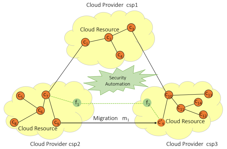
Fig. 1: Illustrative example of security automation for supporting the migration of a resource, noted c_9 , in a cloud composite service, using two exogenous security functions, noted f_1 and f_2
