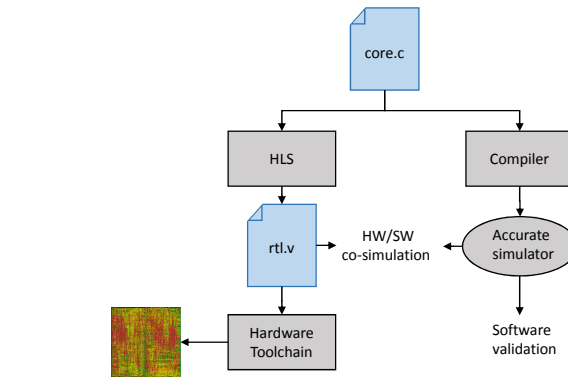
Fig. 1. Comet processor design flow.
