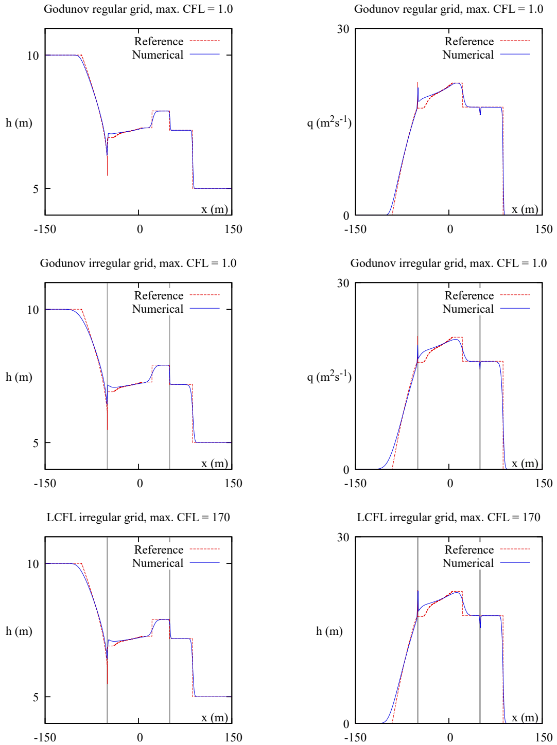
Figure 7: Dambreak problem over sinusoidal bottom. Top: solution computed by the Godunov scheme over a regular grid. Middle: solution computed by the Godunov scheme over an irregular grid with two narrow cells at x = \pm 50 m. Bottom: solution computed by the LCFL method over an irregular grid with two narrow cells at x = \pm 50 m. The locations of the narrow cells are indicated by the vertical grey lines in the middle and bottom graphs.
