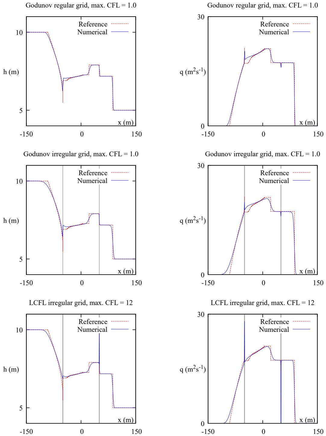
Figure 10: Dambreak problem over discontinuous 32 bottom. Top: solution computed by the Godunov scheme over a regular grid. Middle: solution computed by the Godunov scheme over an irregular grid with two narrow cells \Delta x_1 = 0.1 m at x = \pm 50 m. Bottom: solution computed by the LCFL method over an irregular grid with two narrow cells at x = \pm 50 m. The locations of the narrow cells are indicated by the vertical grey lines in the middle and bottom graphs.
