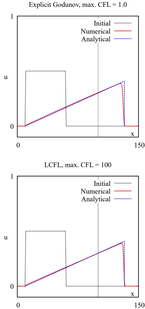
Figure 5: Burgers equation. The narrow cell ( x = 100 m) is indicated by the vertical grey lines in the graphs.
