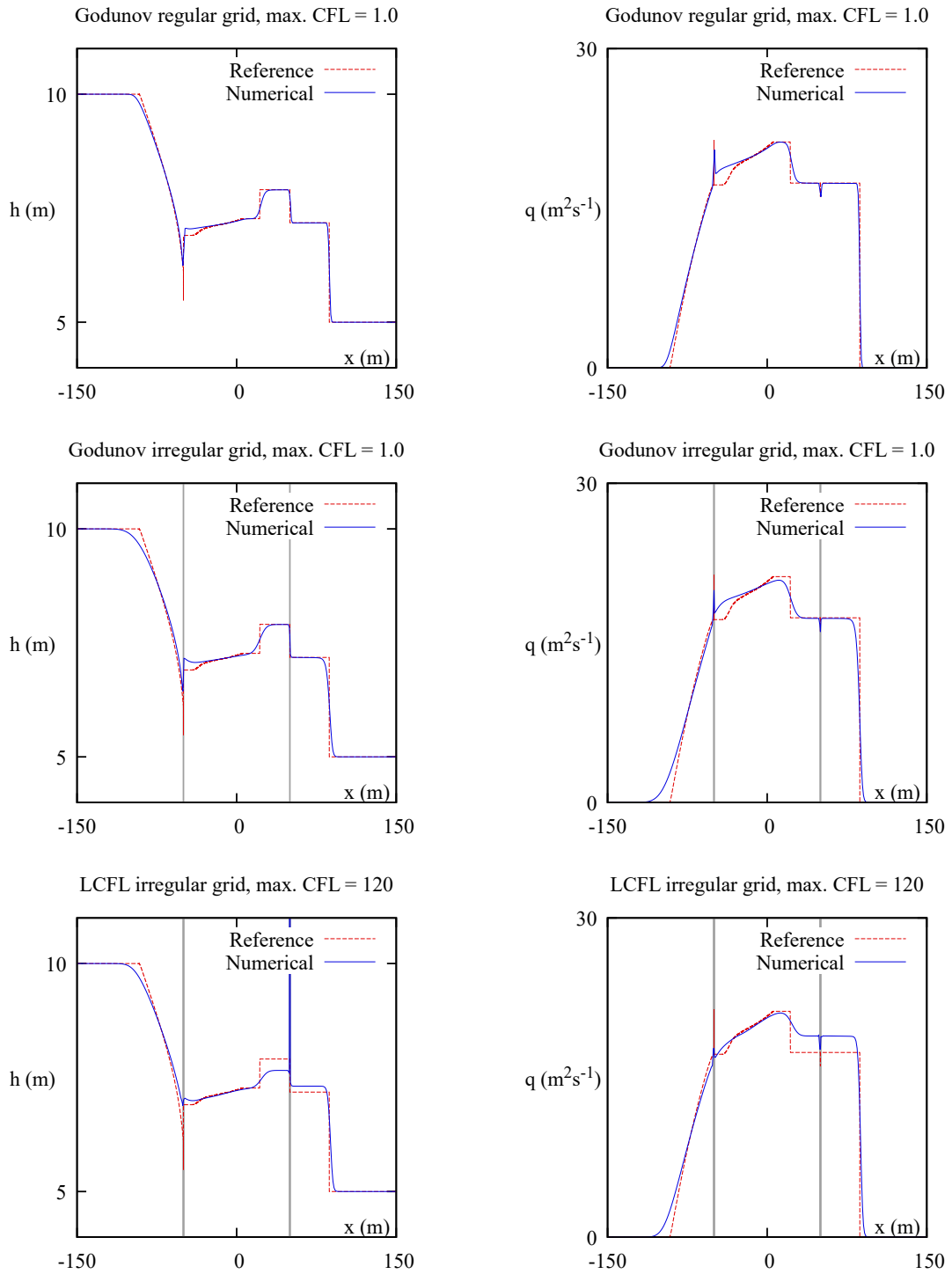
Figure 9: Dambreak problem over discontinuous 31 bottom. Top: solution computed by the Godunov scheme over a regular grid. Middle: solution computed by the Godunov scheme over an irregular grid with two narrow cells \Delta x_1 = 10^{-2} m at x = \pm 50 m. Bottom: solution computed by the LCFL method over an irregular grid with two narrow cells at x = \pm 50 m. The locations of the narrow cells are indicated by the vertical grey lines in the middle and bottom graphs.
