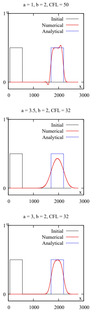
Figure 13: Linear advection equation. Solution for kernel function f^{(2)} . Max. permissible CFL values: 50.27 (top), 34.98 (middle), 37.27 (bottom).
