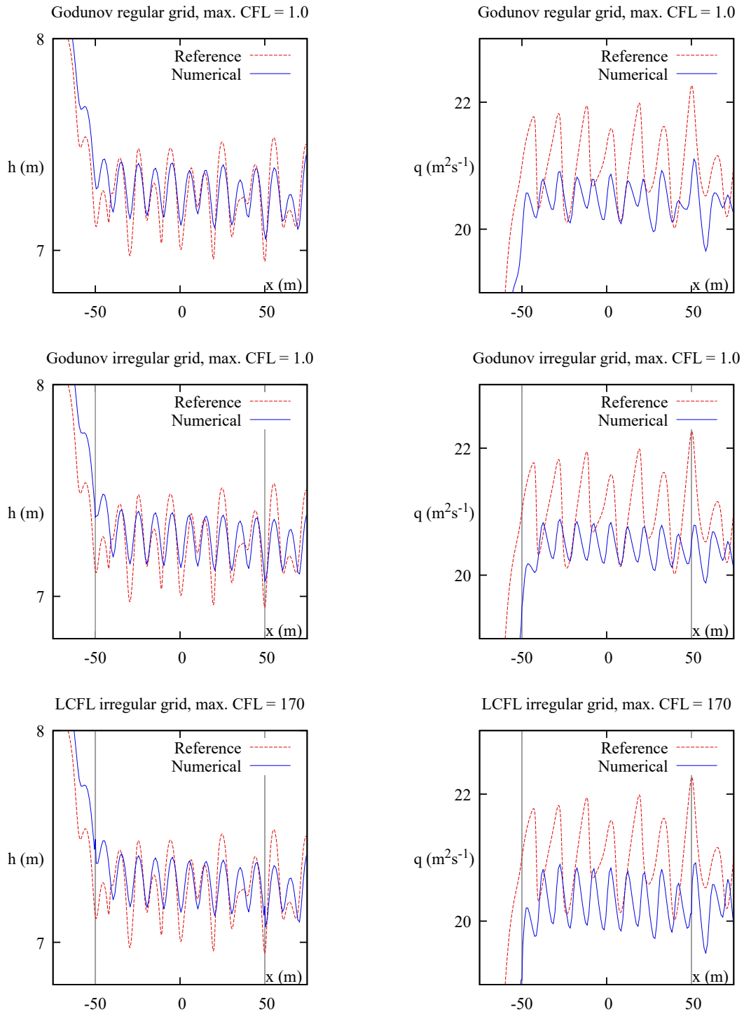
Figure 8: Dambreak problem over sinusoidal bottom 30 . Zoomed graphs over the central parts. Top: solution computed by the Godunov scheme over a regular grid. Middle: solution computed by the Godunov scheme over an irregular grid with two narrow cells at x = \pm 50 m. Bottom: solution computed by the LCFL method over an irregular grid with two narrow cells at x = \pm 50 m. The locations of the narrow cells are indicated by the vertical grey lines in the middle and bottom graphs.
