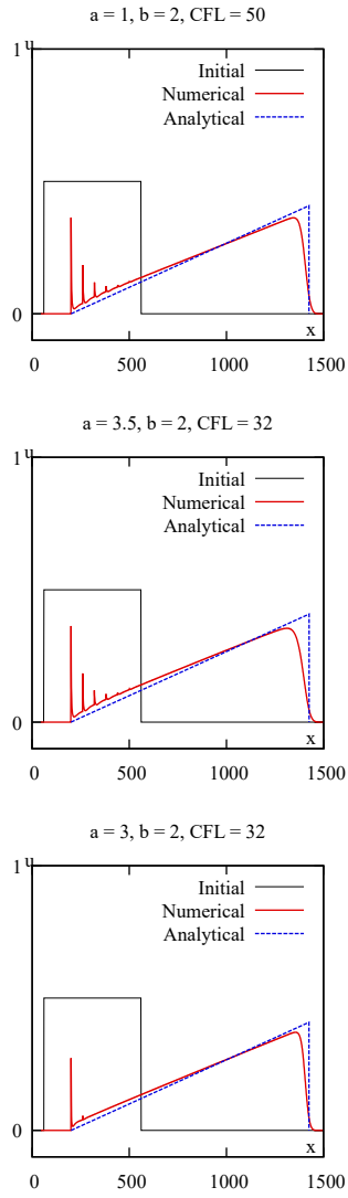
Figure 16: Burgers equation. Solution for kernel function f^{(2)} .
