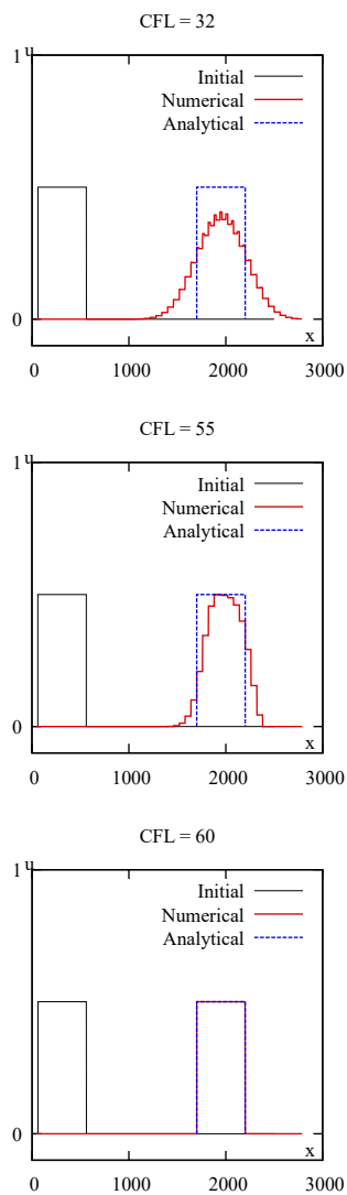
Figure 12: Linear advection equation. Solution for kernel function f^{(1)} . Max. permissible CFL value: 60.
