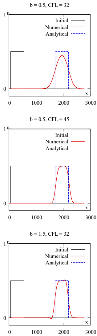
Figure 14: Linear advection equation. Solution for kernel function f^{(3)} . Max. permissible CFL values: 47.62 (top, middle), 33.86 (bottom).
