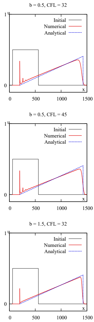
Figure 17: Burgers equation. Solution for kernel function f^{(3)} .
