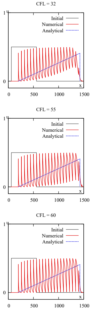
Figure 15: Burgers equation. Solution for kernel function f^{(1)} .
