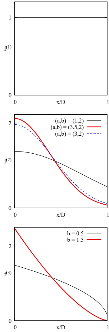
Figure 11: Sample simulations. Kernel functions for the parameters in Table 9
