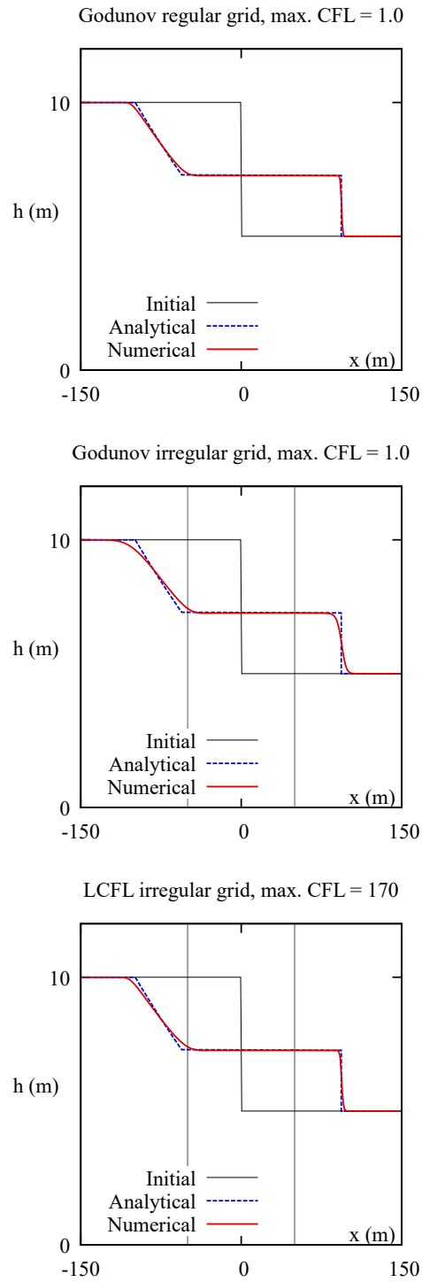
Figure 6: Dambreak problem. Top: solution 28 computed by the Godunov scheme over a regular grid. Middle: solution computed by the Godunov scheme over an irregular grid with two narrow cells at x = \pm 50 m. Bottom: solution computed by the LCFL method over an irregular grid with two narrow cells at x = \pm 50 m. The locations of the narrow cells are indicated by the vertical grey lines in the middle and bottom graphs.
