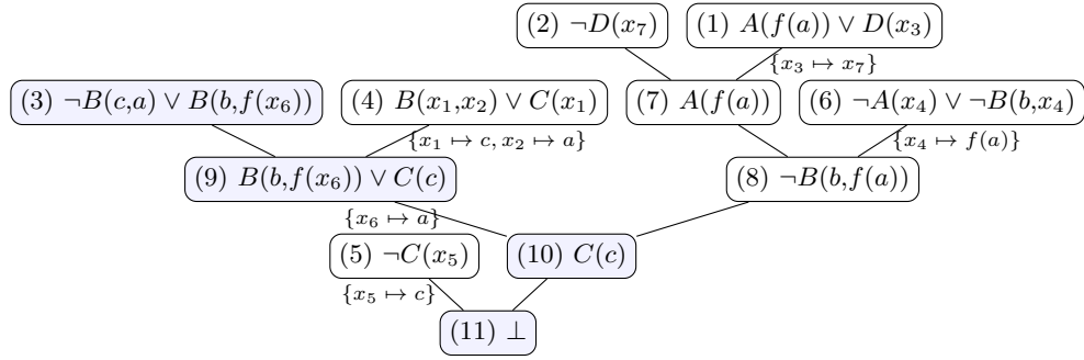
Fig. 1. A refutation of N in tree representation
