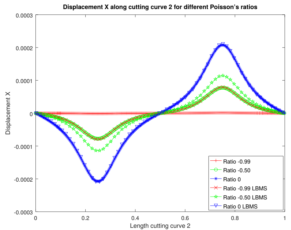
Figure A6. First displacement components along cutting curve C_2 for negative Poisson's ratios.
