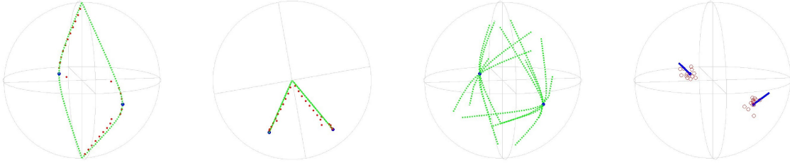
Figure 2. From left to right. (a), (b), Steps 2, 3: one direction ((0, x_3)) , Q = 2 sources (blue), theoretical singularities (green), estimated poles (red); (c), Step 3: theoretical singularity lines cross at sources locations; (d), Step 4: clustering of estimated positions (red), last least-square locations and moments tuning (blue).
