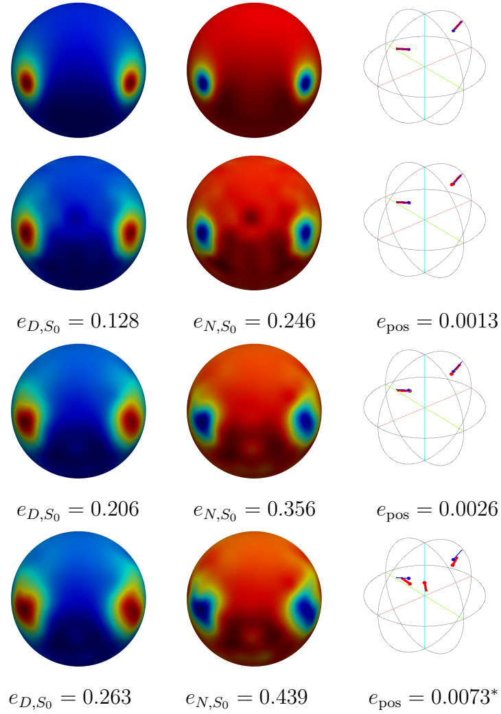
Figure 13. Two distant sources (\mathbf{c}_{q_d}, \mathbf{p}_{q_d}) and (\mathbf{c}_{q-d}, \mathbf{p}_{q-d}) , head model (a): QR reconstruction on the cortex with 257 electrodes and source reconstruction with FS3D. From top to bottom: exact solution, then reconstruction with 0%, 5% and 20% noise. From left to right: Dirichlet trace, Neumann trace, source reconstruction with FS3D.
