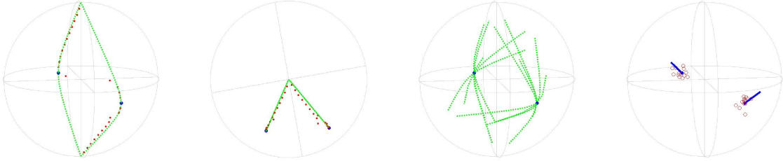
Figure 3. From left to right. (a), (b), Step 3: one direction, Q = 2 sources (blue), theoretic singularities (green), estimated poles (red); (c), (d): (c), Step 3, theoretic singularities lines cross at sources locations; (d), Step 4, clustering of estimated positions (red), last least-square locations and moments tuning (blue).
