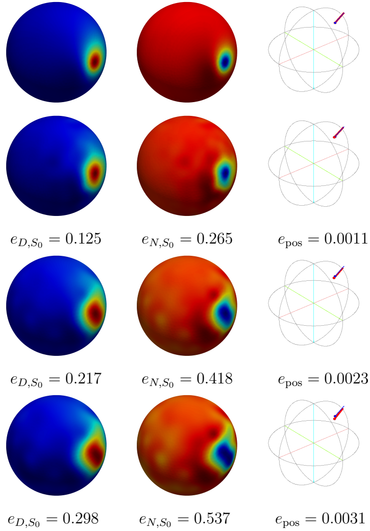
Figure 12. One distant source (\mathbf{c}_{q_d}, \mathbf{p}_{q_d}) and head model (a): QR reconstruction on the cortex with 257 electrodes and source reconstruction with FS3D. From top to bottom: exact solution, then reconstruction with 0%, 5% and 20% noise. From left to right: Dirichlet trace, Neumann trace, source reconstruction with FS3D.
