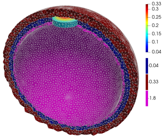
Figure 15. Mesh of the three conductivity regions around the cortex corresponding to CSF, skull and scalp, including the main fontanel region with varying conductivity.
