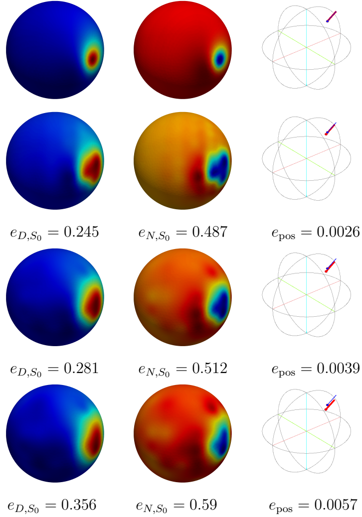
Figure 11. One distant source ( \mathbf{c}_{q_d}, \mathbf{p}_{q_d} ) and head model (a): QR reconstruction on the cortex with 61 electrodes and source reconstruction with FS3D. From top to bottom: exact solution, then reconstruction with 0%, 5% and 20% noise. From left to right: Dirichlet trace, Neumann trace, source reconstruction with FS3D.
