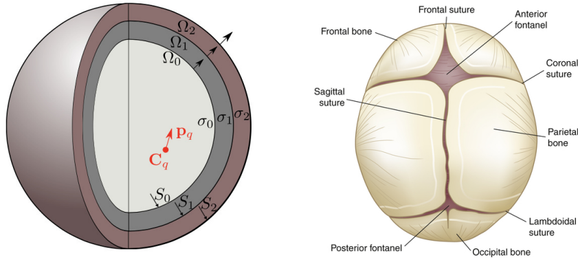
Figure 1. Left: Spherical head model with L = 3 and one source (\mathbf{c}_q, \mathbf{p}_q) . Right: Fontanels and skull of a neonate.
