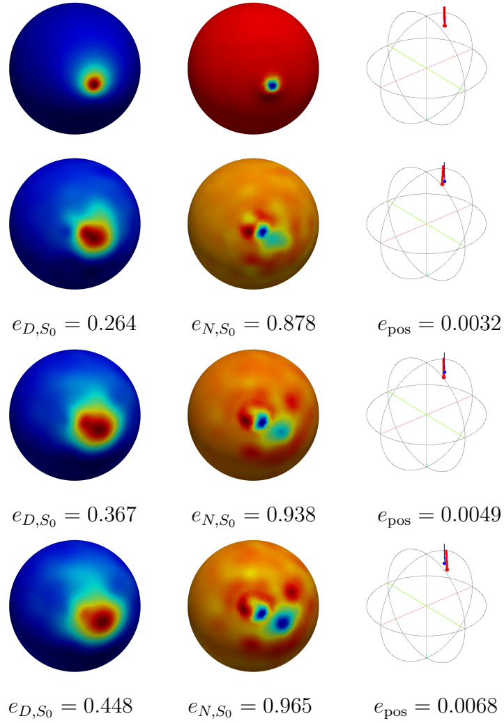
Figure 16. One close source (\mathbf{c}_{q_c}, \mathbf{p}_{q_c}) , model (b) with CSF and fontanel: QR reconstruction on the cortex with 257 electrodes and source reconstruction with FS3D. From top to bottom: exact solution, then reconstruction with 0%, 5% and 20% noise. From left to right: Dirichlet trace, Neumann trace, source reconstruction with FS3D.
