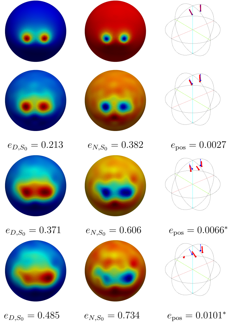
Figure 14. Two close sources (\mathbf{c}_{q_c}, \mathbf{p}_{q_c}) and (\mathbf{c}_{q_{-c}}, \mathbf{p}_{q_{-c}}) and head model (a): QR reconstruction on the cortex with 257 electrodes and source reconstruction with FS3D. From top to bottom: exact solution, then reconstruction with 0%, 5% and 20% noise. From left to right: Dirichlet trace, Neumann trace, source reconstruction with FS3D.
