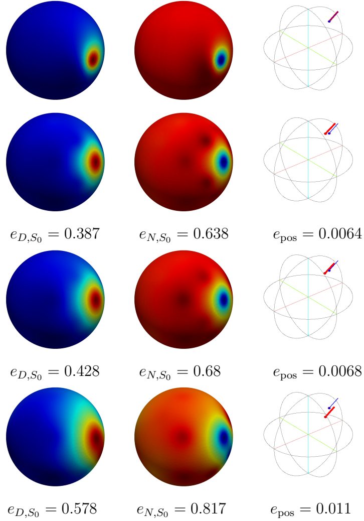
Figure 10. One distant source ( \mathbf{c}_{q_d}, \mathbf{p}_{q_d} ) and head model (a): QR reconstruction on the cortex with 33 electrodes and source reconstruction with FS3D. From top to bottom: exact solution, then reconstruction with 0%, 5% and 20% noise. From left to right: Dirichlet trace, Neumann trace, source reconstruction with FS3D.
