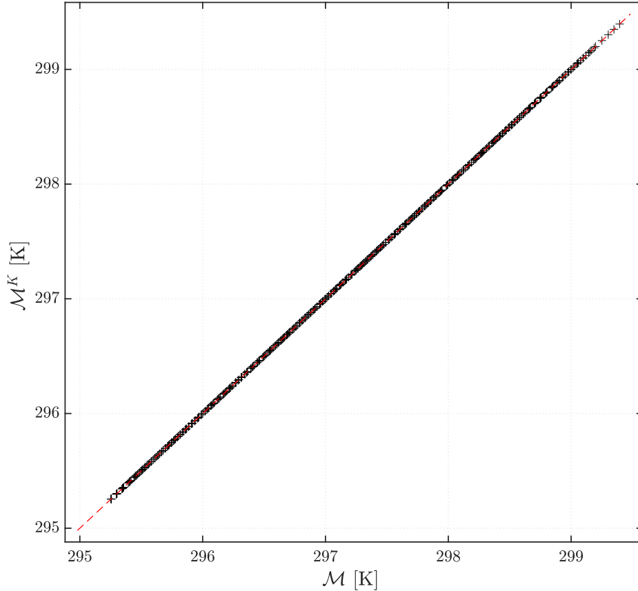
Figure 6: Comparison of surrogate model evaluations of temperature \mathcal{M}^K with the CFD model \mathcal{M} for given inputs \mathbf{R}^{(i)} . The red line represents the first bisector curve.
