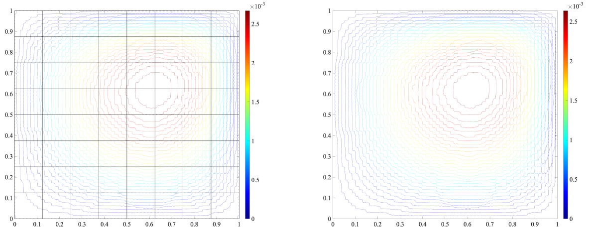
FIGURE 4. Isolines of the MHM solution overlaid with the rectangular mesh with 64 squares (left) alongside the reference solution (right). Here \epsilon = \frac{1}{64} , \ell = 1 and h = H .
