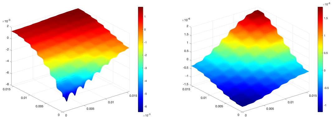
FIGURE 1. A typical multiscale basis function (left) and \widehat{T}_\varepsilon f (right) on a quadrangular element of \mathcal{T}_H . Here \varepsilon = \frac{1}{64} and \ell = 1 .
