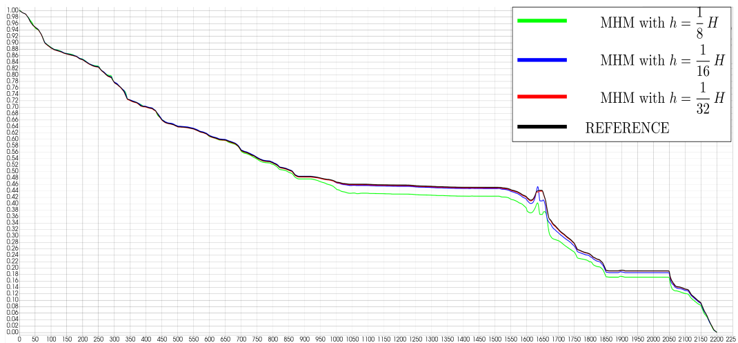
FIGURE 7. Comparison of the profiles at the x_1 = 199 between three MHM solutions obtained different levels of refinement on edges and the reference solution. Here \ell = 1 .
