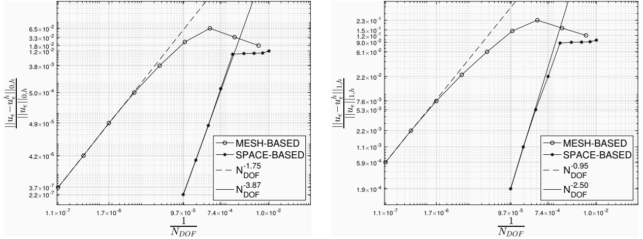
FIGURE 3. Convergence history with respect to N_{DOF} in the relative L^2(\Omega) (left) and H^1(\mathcal{T}_H) (right) norms. Comparison between the one piecewise linear interpolation per edge case with mesh refinement (mesh-based) and the multiple piecewise linear interpolation per edge case on a fixed mesh (space-based). The latter induces a tremendous improvement in the quality of the numerical results with fewer degrees of freedom.
