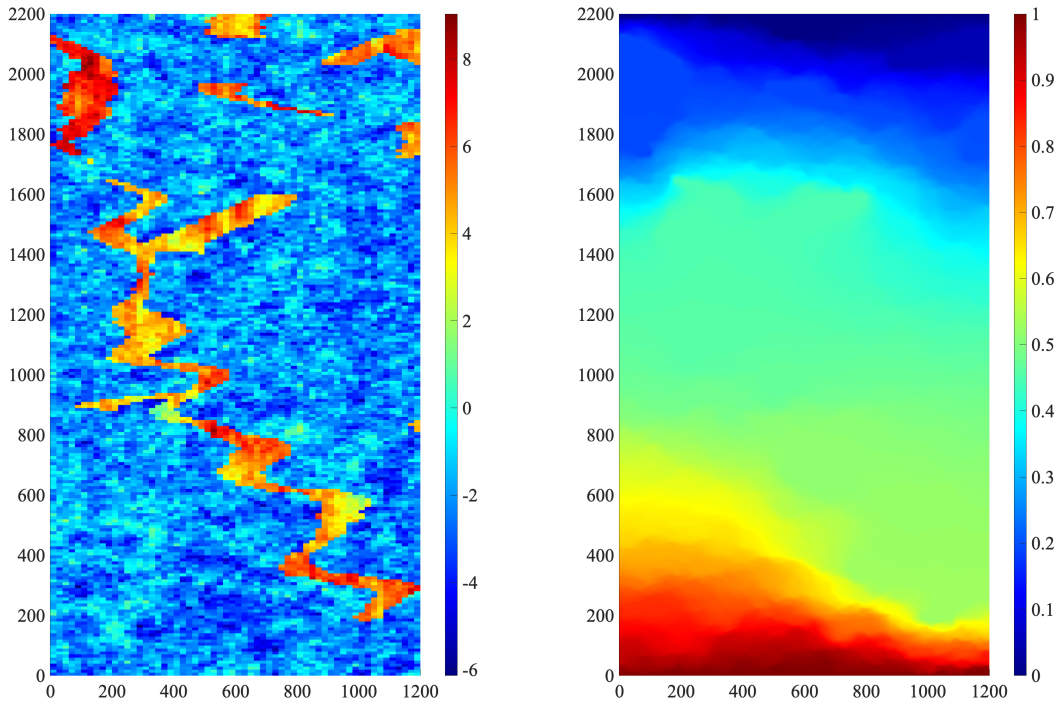
FIGURE 5. Logarithm of the permeability proposed in [22] (left) and the isolvalues of the reference solution (right).
