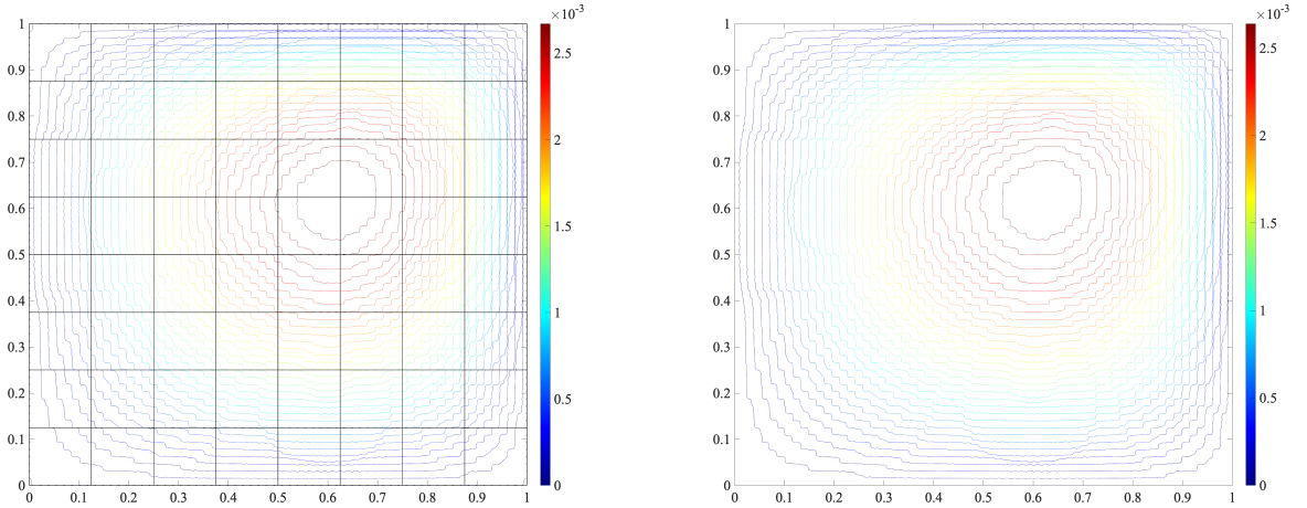
FIGURE 4. Isolines of the MHM solution overlaid with the rectangular mesh with 64 squares (left) alongside the reference solution (right). Here \varepsilon = \frac{1}{64} , \ell = 1 and h = H .
