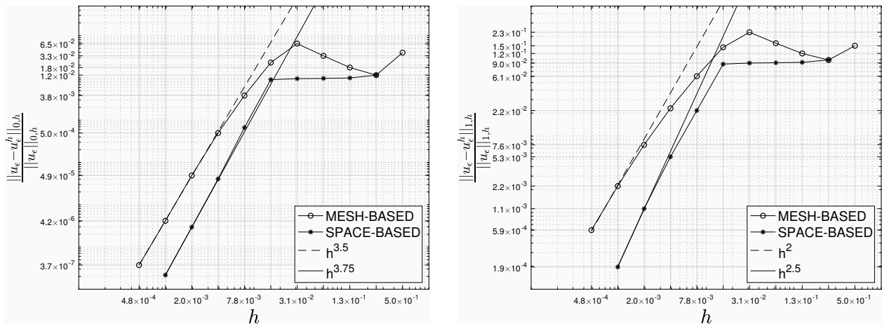
FIGURE 2. Convergence history with respect to h in the relative L^2(\Omega) (left) and H^1(\mathcal{T}_H) (right) norms. Comparison between the one piecewise linear interpolation per edge case with mesh refinement (mesh-based) and the multiple piecewise linear interpolation per edge case on a fixed mesh (space-based).
