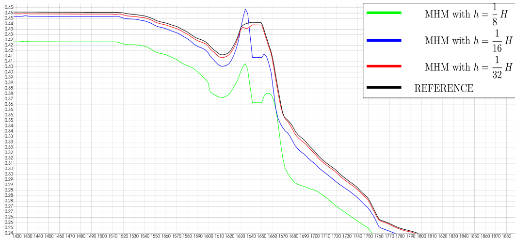
FIGURE 8. Zoomed solutions in the area around x_2 = 1,650 in Figure 7.
