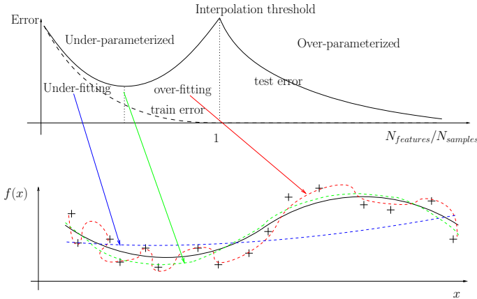
Fig. 1 Double descent “paradox”. On the left is the traditional picture of a U-shape curve of the test error showing first under-fitting corresponding to high bias, followed by over-fitting characterized by high variance as illustrated on the 1-d regression problem. The right part corresponds often to the deep learning setting with high complexity/expressivity of the model along with low test error (Color figure online)
