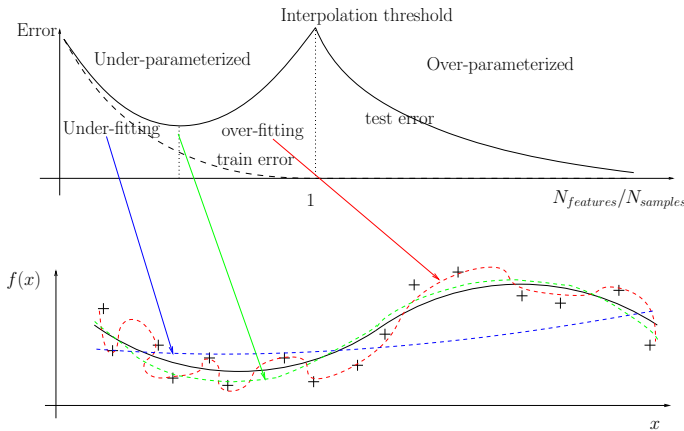
Fig. 1 Double descent “paradox”. On the left is the traditional picture of a U -shape curve of the test error showing first under-fitting corresponding to high bias, followed by over-fitting characterized by high variance as illustrated on the 1-d regression problem. The right part corresponds often to the deep learning setting with high complexity/expressivity of the model along with low test error (Color figure online)
