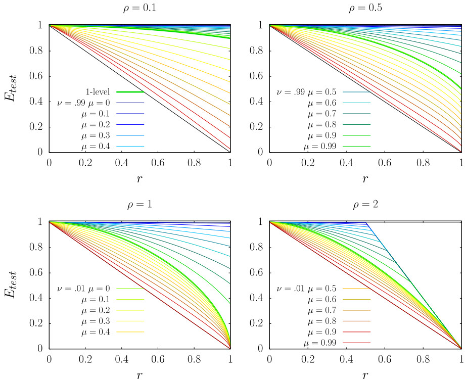
Fig. 4 The optimal performance in terms of E_{\text{test}} of the 2-level model as a function of r , depending on the fraction \nu of strong modes and on the fraction \mu of longitudinal spectral power of the signal on these modes. The performance of the 1-level model defines the frontier between the aligned and anti-aligned domains, represented here respectively by the \nu = 0.01 and \nu = 0.99 set of curves (Color figure online)
