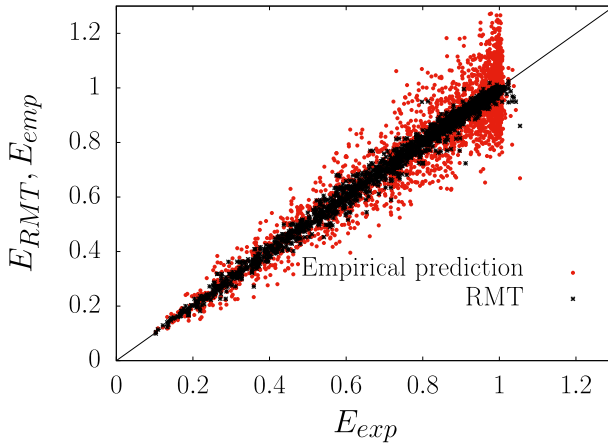
Fig. 3 Scatter plot of the test error E_{\text{exp}} measured on experiments done with a two 2-level population matrix model with eigenvalues \{1, 50\} , versus the expected results (3.19) from RMT and the empirical prediction (3.23) obtained from the training. The experimental point are obtained with a train set of size N_s = 200 and test set of size 10^4 . By convenience, the default coupling is set to \alpha = \alpha^* delivered by the RMT, \rho is varied \in \{0.5, 1.0, 2.0\} , \nu \in \{0.01, 0.99\} and \mu \in [0, 1] (Color figure online)
