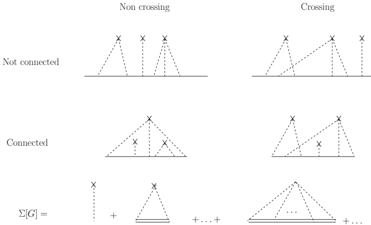
Fig. 8 Examples of Feynman Diagrams corresponding to a contribution proportional to \rho^3 \tau^6 . The plain line represents the propagator line and corresponds to insertion of the free propagator G_0(z) between two successive interaction lines (dotted lines) or edges. The top left one for instance is -\rho^3 \mathbb{E} \left[ G_0 \omega_1 \omega_1^t G_0 \omega_1 \omega_1^t G_0 \omega_2 \omega_2^t G_0 \omega_3 \omega_3^t G_0 \omega_3 \omega_3^t G_0 \omega_3 \omega_3^t G_0 \right] , and is both non-crossing and not connected. The double plain line corresponds to use the full propagator instead in the expansion of the free energy
