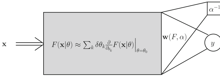
Fig. 5 Schematic plot of the regression model considered here. The weight vector \mathbf{w}(F, \alpha) of the last layer solves a ridge regression with penalty \alpha^{-1} depending on the vector of features functions F(\mathbf{x}|\theta) defined by some NN with parameters \theta represented by the grey box. In the “semi-lazy” regime F(\mathbf{x}|\theta) is taken close to some reference parameter \theta_0 , with \delta\theta = \theta - \theta_0
