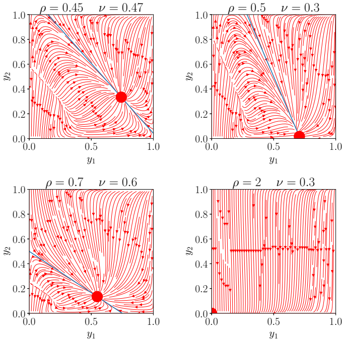
Fig. 7 Examples of phase portraits corresponding to the autonomous system (4.25, 4.26). The red dot locate the stable fixed point while the blue line represents \Lambda(y_1, y_2) = 0 given by (4.21) above which is the valid domain \mathbb{D} (Color figure online)
