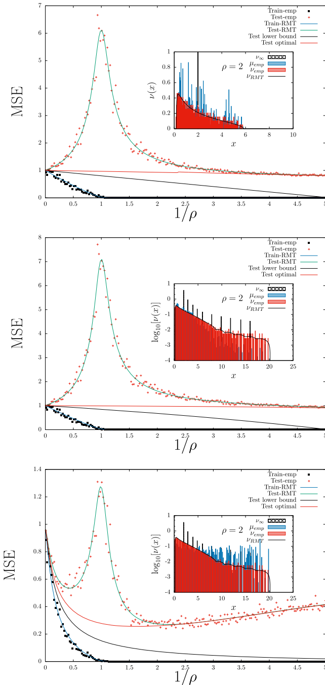
Fig. 2 Main plots: Test and train error as a function of \rho^{-1} given by RMT (plain lines) and a single experiments with N = 200 , when the population matrix has one degenerate level (top panel) and ten degenerate levels, with wrong alignment (middle panel) and good alignment (bottom panel) of the signal with the population matrix. Inset: spectral densities of the population (in gray), empirical feature matrices (in red) and spectral power of the signal on the corresponding levels (blue) (Color figure online)
