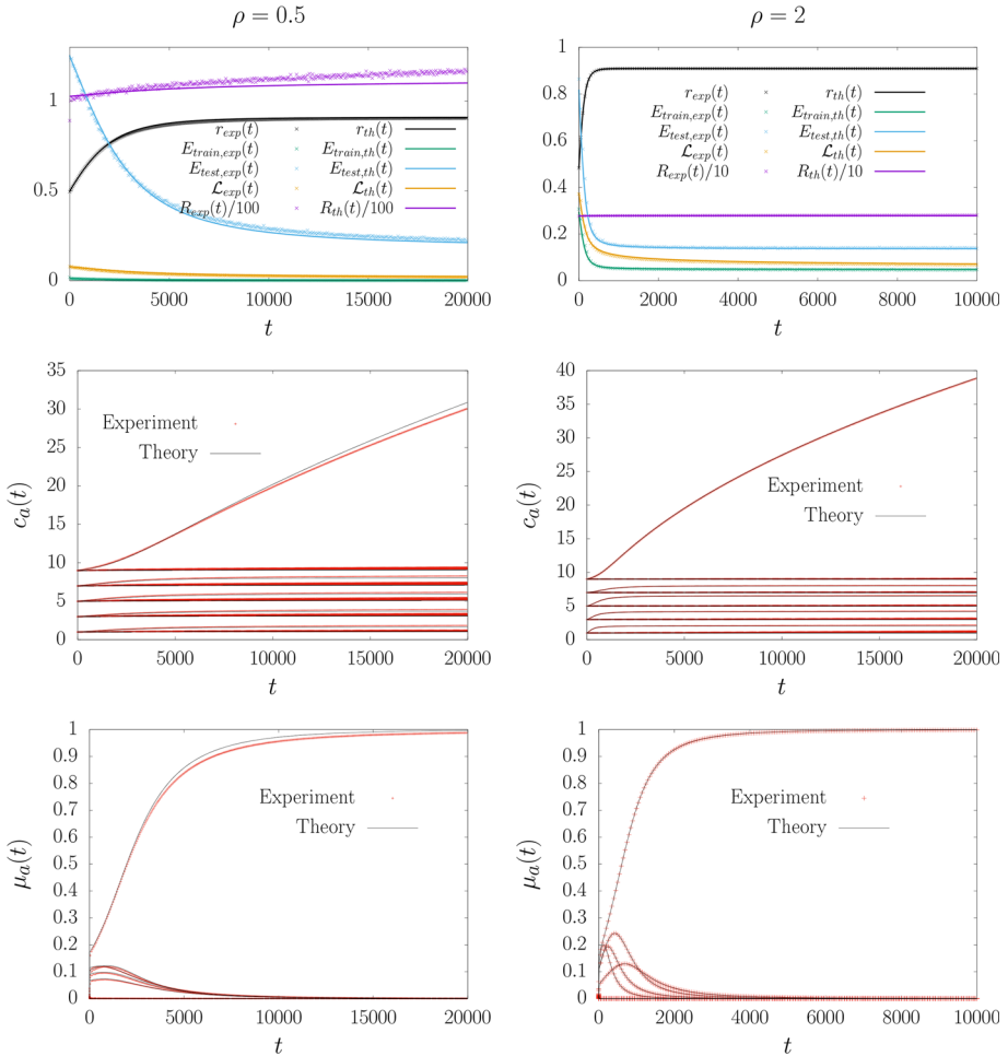
Fig. 6 Feature learning process dynamics: comparison between actual feature learning processes and the corresponding dynamical system (4.10, 4.11). The left and right panels are respectively in the over- and under-parameterized regime with same level of noise \sigma^2 = 0.1 . The population matrix is initialized with 5 equally spaced and degenerate levels. Concerning the learning process we have in both cases N_f = D/2 = 100 (Color figure online)
