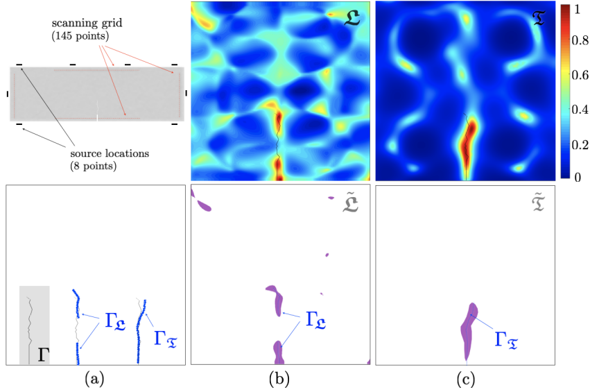
Figure 2: Time- vs. frequency- domain reconstructions from post-fracturing data: (a-top) sensing configuration, (a-bottom) ground truth \Gamma compared against the recovered \Gamma_{\Xi} and \Gamma_{\tilde{\Xi}} obtained from the thresholded maps, (b) multifrequency indicator map \Xi and its 60% thresholded counterpart \tilde{\Xi} [22], and (c) time-domain indicator map \Xi (6.24) and its affiliated \tilde{\Xi} (6.25) thresholded at 60%.
