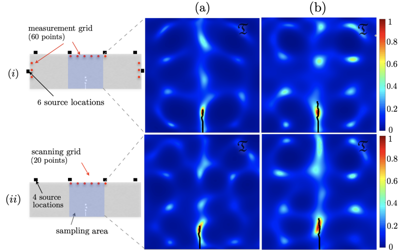
Figure 5: Partial-aperture time-domain reconstruction via (6.24) at (a) 90% and (b) 75% of the maximum load. The loci and number of source/measurement points (for each case) is indicated in the left column.
