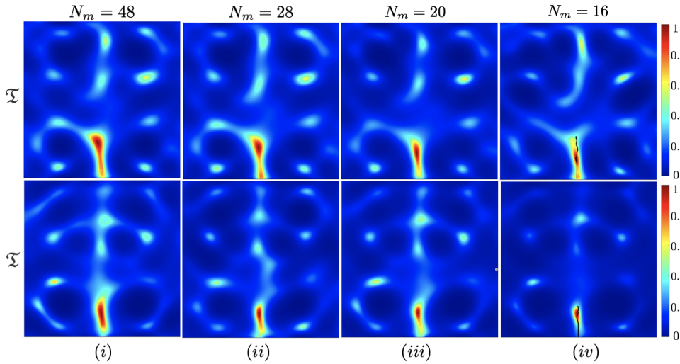
Figure 3: Time-domain reconstruction from reduced data at 75% (top) and 90% (bottom) of the maximum load where \Gamma_m is sampled by N_m points.
