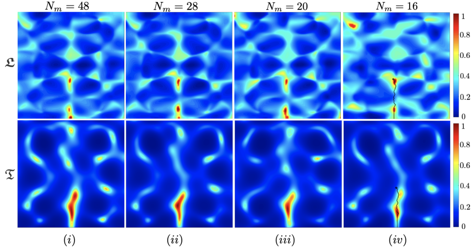
Figure 4: Time- vs. frequency- domain inversion from reduced data at 60% of the maximum load: (top) multifrequency indicator \mathfrak{L} [22], and (bottom) time-domain indicator \mathfrak{T} . Here, the number of scanning points on \Gamma_m is N_m .
