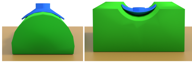
Fig. 11. Two curved surfaces presented in Figure 10 (last on the right) when the suction cup is flattened onto the object, showing that no sealed cavity can be created between them due to the design of the cup.
