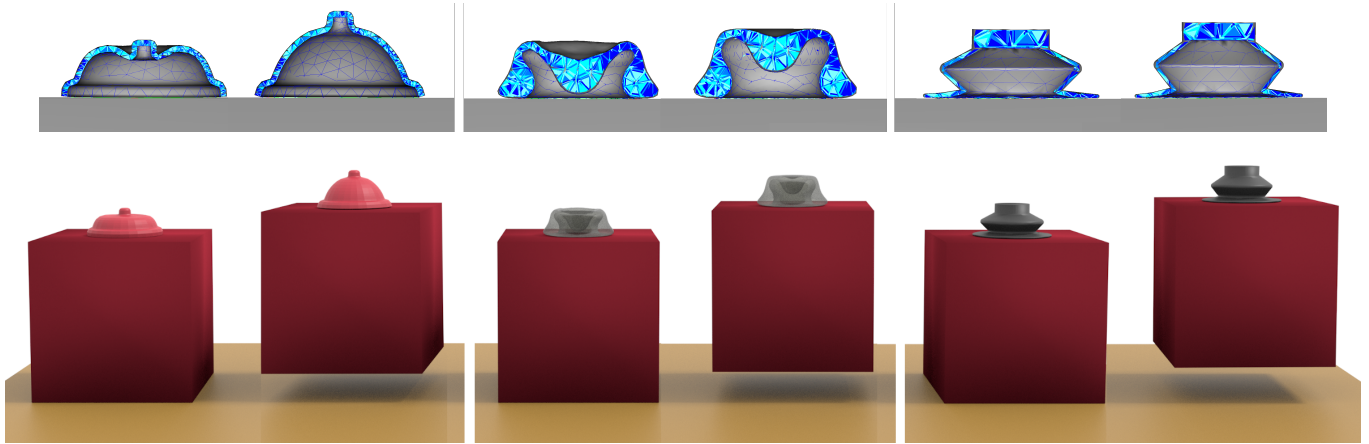
Fig. 12. Three suction cups with different shape succeeding at lifting a rigid cube of 190 g. Top: clipped views showing the shape of the three cups. The gray triangles show the surface mesh used for visualization, and the blue elements show the volume tetrahedral mesh used for the FEM model. Bottom: corresponding global view of the simulation.
