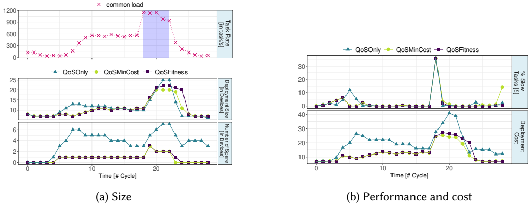
Fig. 9. Comparison of the three algorithm alternatives when handling a 28-hour workload trace (simulator).
