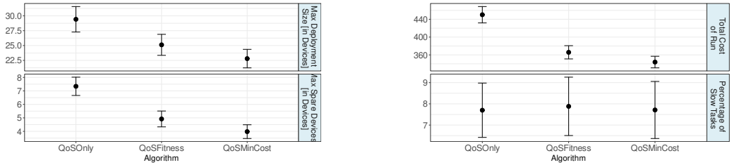
Fig. 10. Analysis of the chosen indicators for a 28-hour workload trace (simulator).
