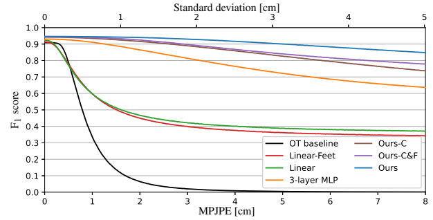
Figure 6: F_1 score on foot contacts detection from motion sequences purposely noised with additive isotropic Gaussian noise. Each curve represents the F_1 score against the amount of noise introduced, measured with the MPJPE in centimeters indicated by the bottom horizontal axis, while the top horizontal axis gives the corresponding standard deviations of the Gaussian noise. The results indicate that our method is more robust to noise.
