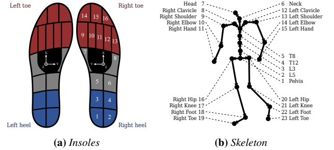
Figure 2: Left) Pressure cell layout of Moticon's OpenGo Sensor Insoles [AG21]. Blue (1 to 4) and red (9 to 16) cells are the groups of cells used to compute heel and toe contacts, respectively. Axes at insole centers represent inertial measurement units (IMUs). Right) Xsens MVN's [SGB18] motion capture skeleton with 23 joints.
