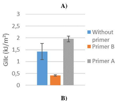
Figure 15 : A) ASTM CRITICAL TOUGHNESS COMPUTATION, B) J-INTEGRAL CRITICAL TOUGHNESS COMPUTATION
