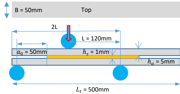
Figure 9: ENF TEST SAMPLE GEOMETRY
