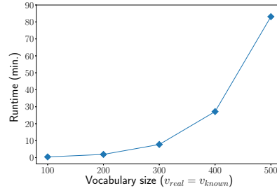
Fig. 7. Runtime of the CKWS-adapted refined score attack using known-documents w.r.t. to vocabulary size, with d = 2 and p = 0.7 .
