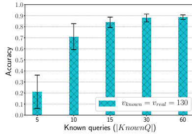
Fig. 4. Accuracy plot of the CKWS-adapted refined score attack with d = 2 and varying number of known queries. With |\mathcal{D}_{real}| = 18K , |\mathcal{D}_{similar}| = 12K , |Q| = 0.15 \cdot m_{real} .
