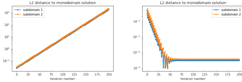
Fig. 1: L^2 distance to monodomain of the solution on each subdomain as a function of the iteration number when using (26) and (27) respectively.
