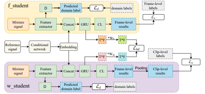
Figure 2: The architecture of the mixed supervised learning framework. CL denotes classification layers, which includes two fully-connected layers and one softmax function. D denotes the discriminator, which consists of three convolutional layers and one fully-connected layer.
