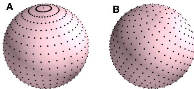
Figure 1: Two types of spatial discretization of points on a sphere. (A) equal-angle and (B) Fibonacci. (A) results in denser points at the poles than at the equator, while (B) does not.
