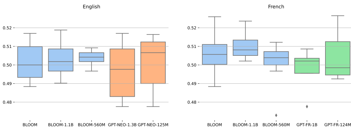
Figure 13: Overall accuracy of BLOOM on crowS-Pairs per prompt for English and French. Results on the two smallest BLOOM models and monolingual GPT models of comparable size are also shown.
