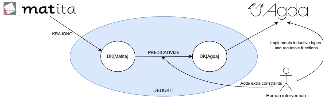
Figure 8 Diagram representing the translation of MATITA's arithmetic library into AGDA
