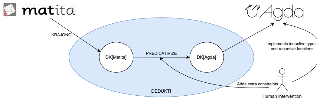
■ Figure 8 Diagram representing the translation of MATITA's arithmetic library into AGDA
