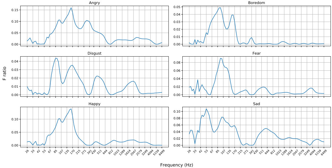
Fig. 4: CWT F-ratio for different frequency bins over EmoDB database.
