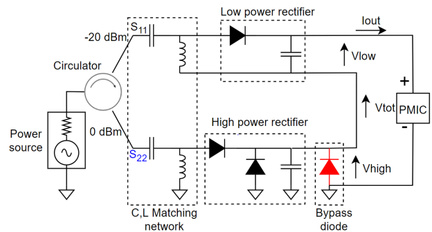
Fig. 3. Series rectifier association with a bypass diode at the output of the high power rectifier.
