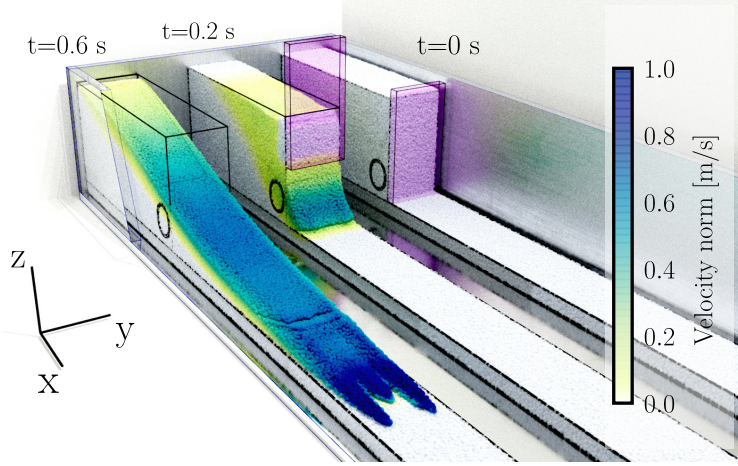
Figure 7: 3D MPM simulations of the B15 granular column collapses over a 15°-tilted bed at three different times. The motion due to the lifting gate is particularly visible at t = 0.2 s. A three-dimensional animated visualisation is provided in the online supplementary material (c.f. movie 3).
