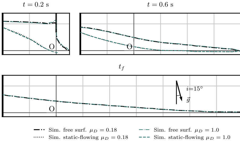
Figure 21: Impact of the lifting gate friction: comparison of simulations of the 15^\circ bead collapse with the standard friction coefficient between the material and the door \mu_D = 0.18 (black lines) and a non-realistic high coefficient \mu_D = 1 (green lines).
