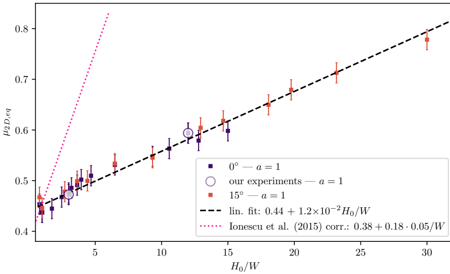
Figure 17: 2D equivalent friction coefficient determined to best match the corresponding 3D final free-surface, as a function of the channel width, for the 0° and 15° beads collapses. Our results seem compatible with a linear dependency, which we illustrate by the dashed fit. We also report the linear scaling (pink dotted line) used by Ionescu et al. (2015).
