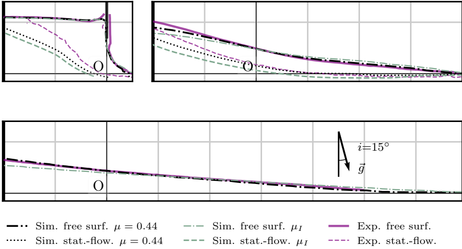
Figure 11: Comparison of 3D simulations performed with \mu = \mu_a = 0.44 (black lines) and \mu = \mu(I) (green lines) for the 15^\circ bead collapse (B15) at t = 0.2 s, 0.6 s and t_f .
