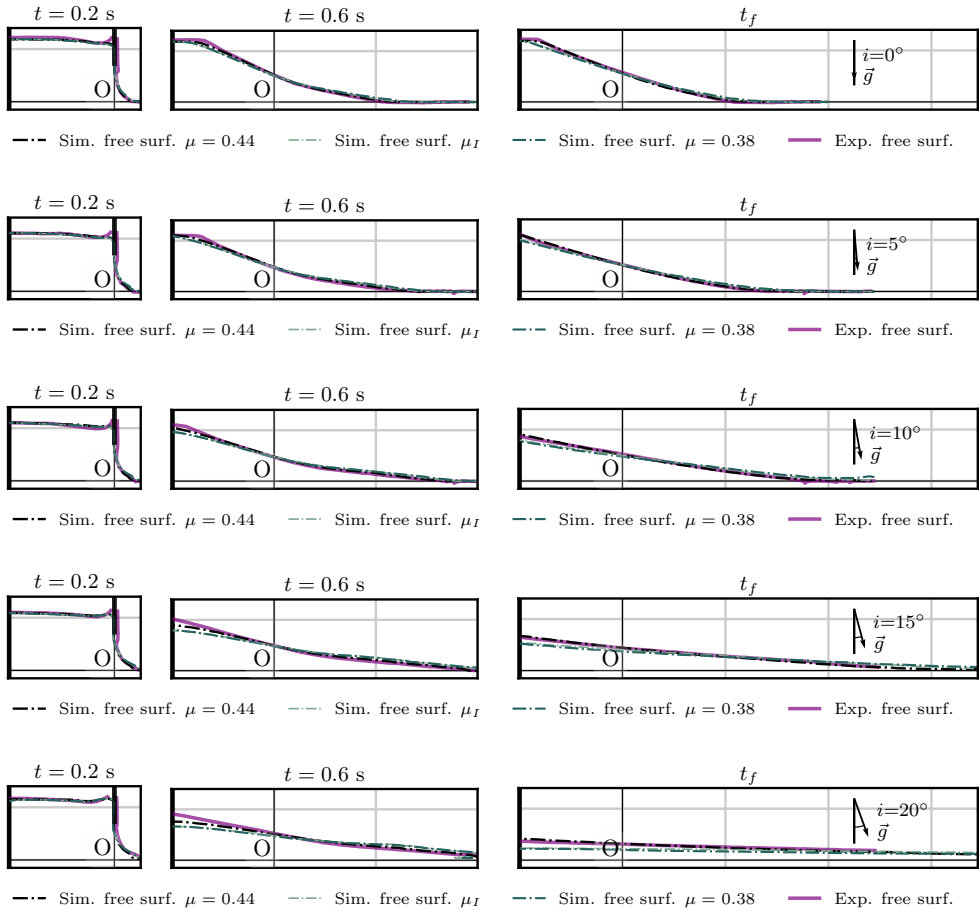
Figure 20: Comparison of 3D simulations performed with \mu = \mu_a = 0.44 (black lines), \mu = \mu(I) and \mu = \mu_{stop} = 0.38 (blue lines) for the all the bead collapses at t = 0.2 s, 0.6 s and t_f . Experimental curves (solid pink line) are provided for reference, and we show both the free-surface lines (resp. plain and dash-dotted) and the static-flowing transition contours (resp. dashed and dotted).
