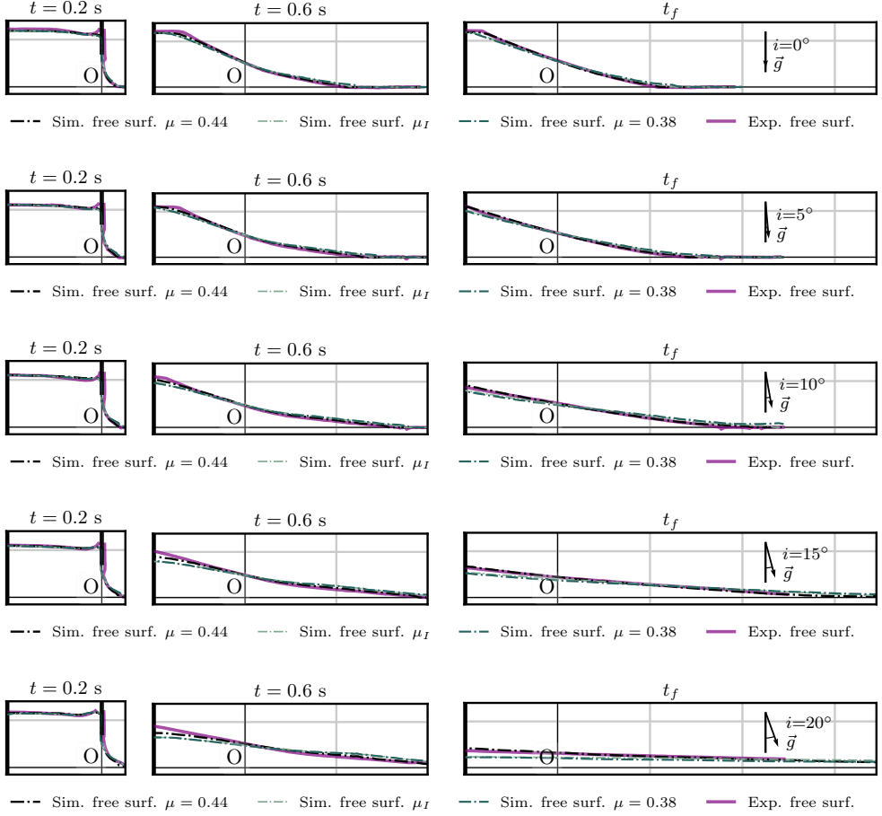
Figure 20: Comparison of 3D simulations performed with \mu = \mu_a = 0.44 (black lines), \mu = \mu(I) and \mu = \mu_s = 0.38 (blue lines) for the all the bead collapses at t = 0.2 s, 0.6 s and t_f . Experimental curves (solid pink line) are provided for reference, and we show both the free-surface lines (resp. plain and dash-dotted) and the static-flowing transition contours (resp. dashed and dotted).
